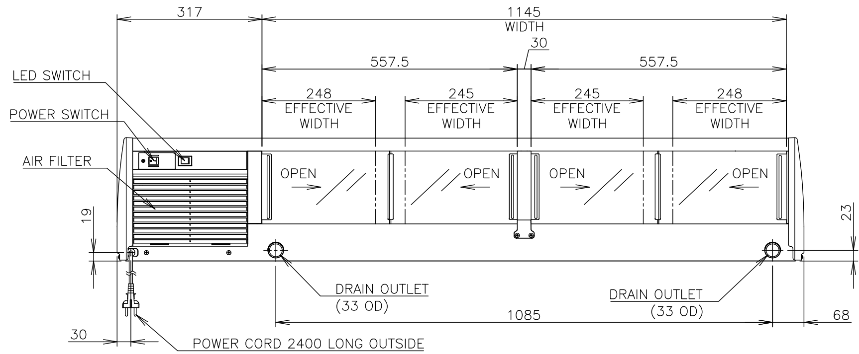
VIEW A(REAR)
