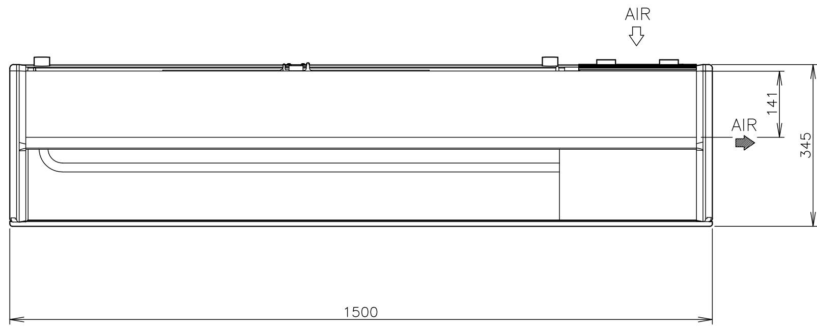
VIEW A(REAR)
