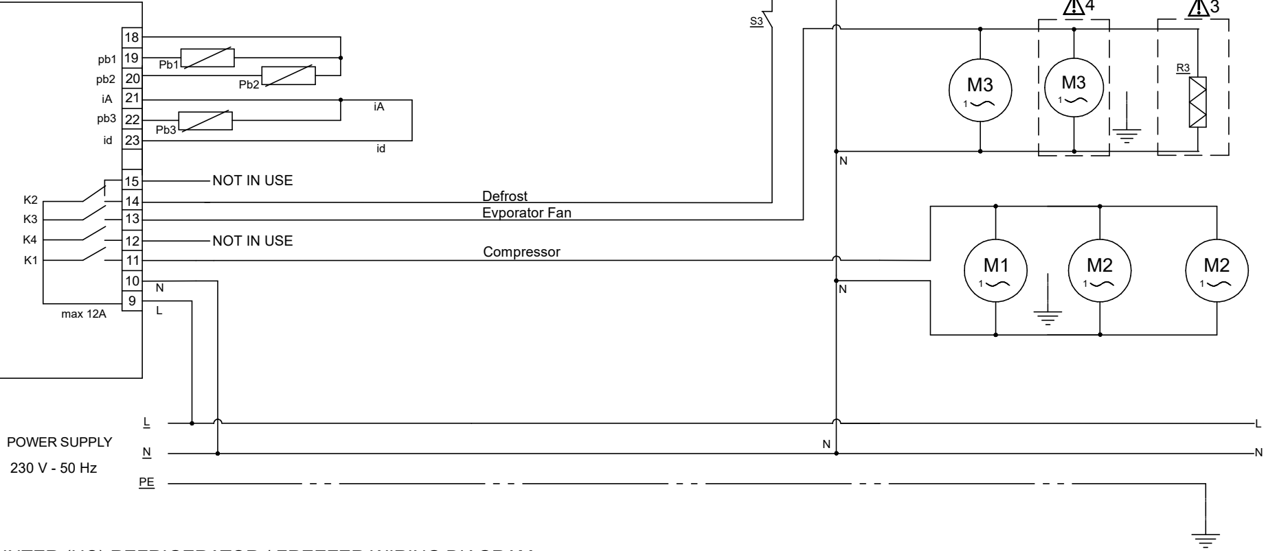
PREMIER UNDERCOUNTER (UC) REFRIGERATOR / FREEZER WIRING DIAGRAM
